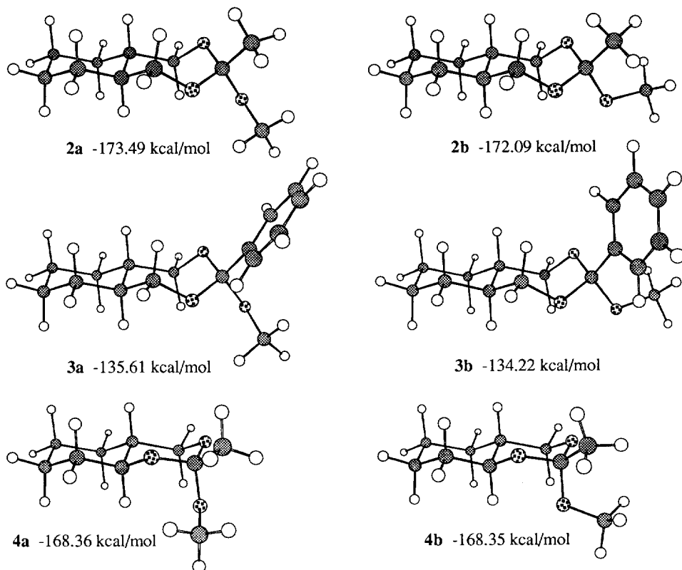
Scheme 5. AM1 optimized structures of the orthoesters 2-4.
