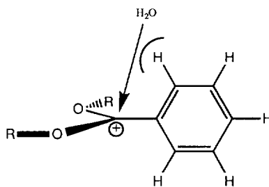
Scheme 8
