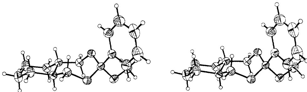
Figure. X-Ray structure of 3b.
