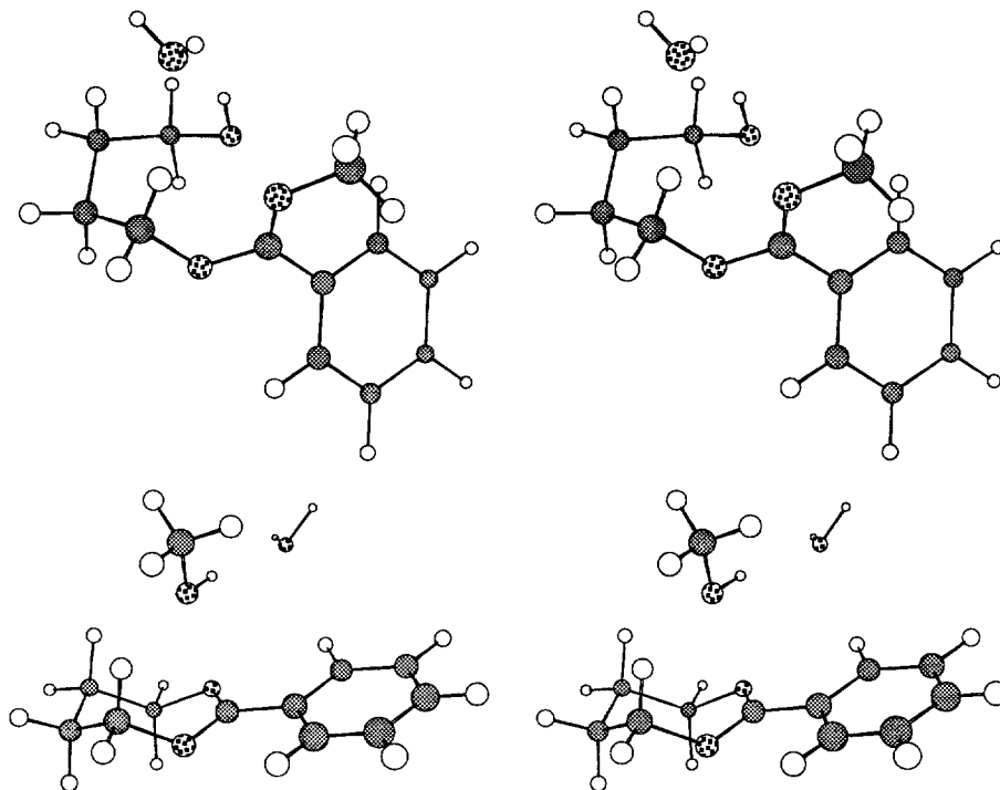
Scheme 7. Cation from 23f (top). Cation from 23a (bottom).
