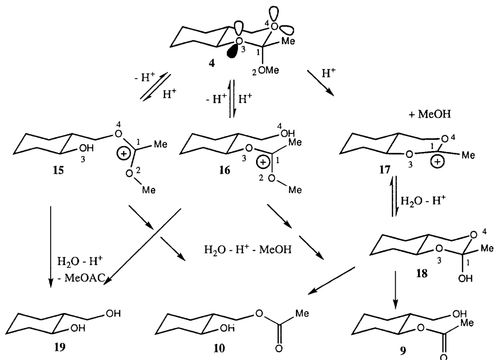
Scheme 4. Hydrolysis pathway for the orthoester 4.
