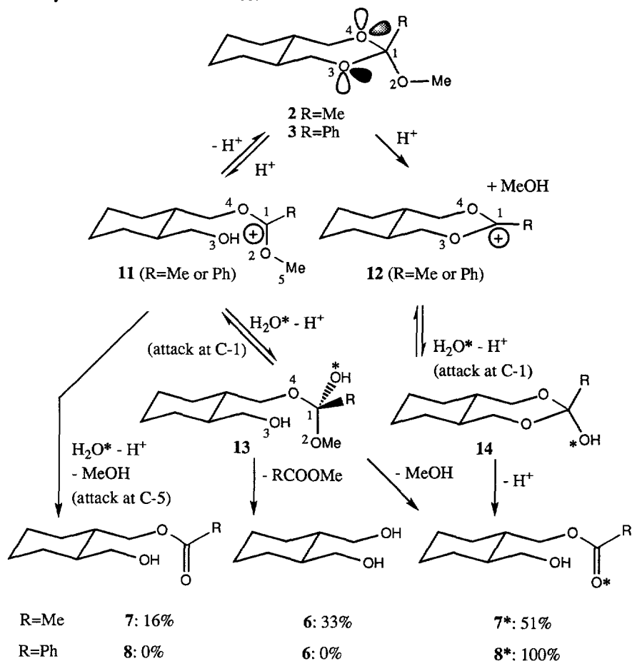
Scheme 3. Hydrolysis pathways for the orthoesters 2 and 3 .
